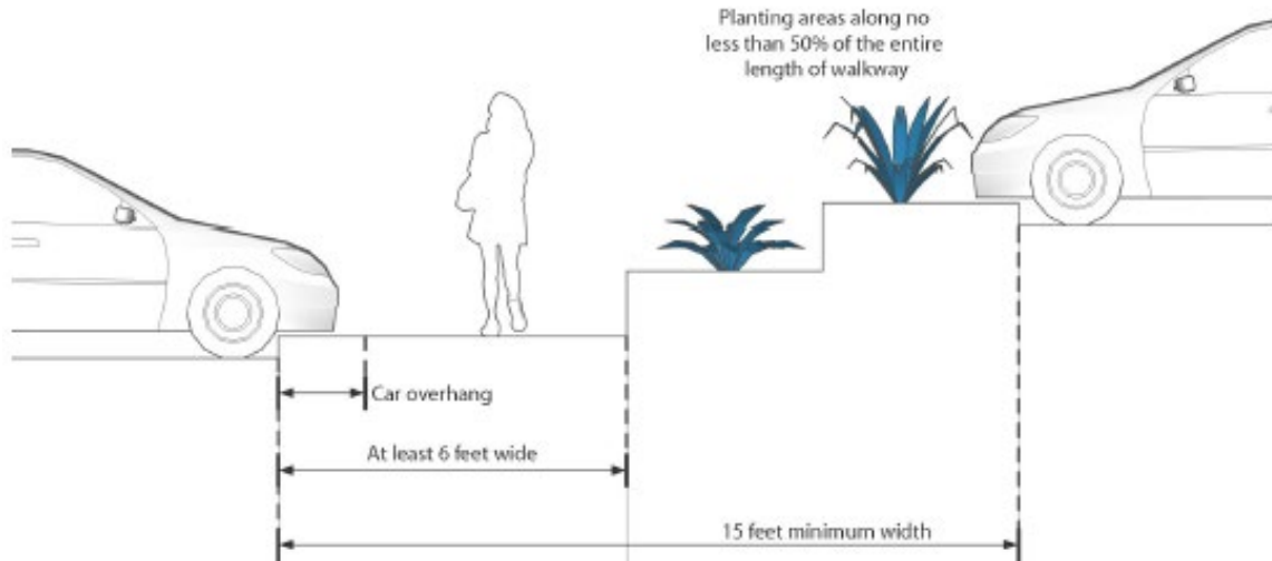
Figure 4-32. Walkway Design
