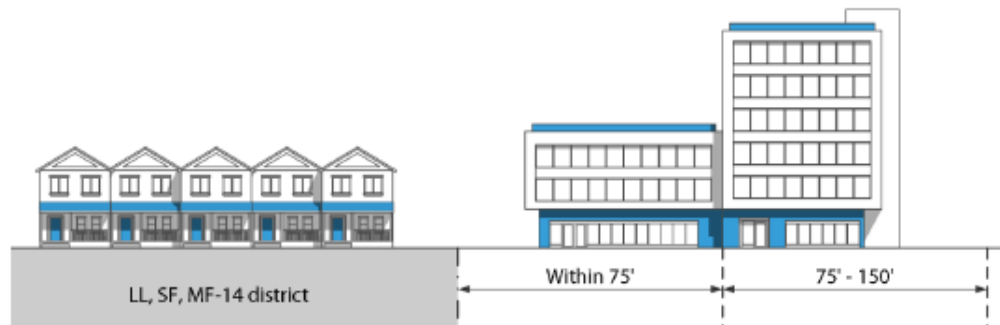
Figure 4-17: Residential Adjacency Stepback and Height Limit
