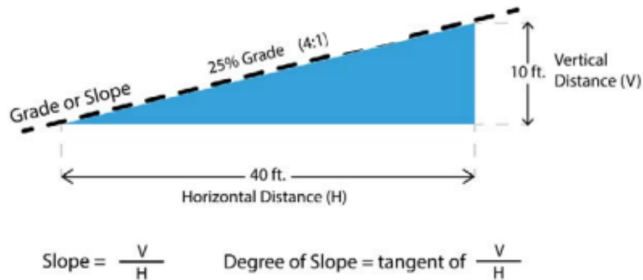
Figure 9-3: Slope Calculation
